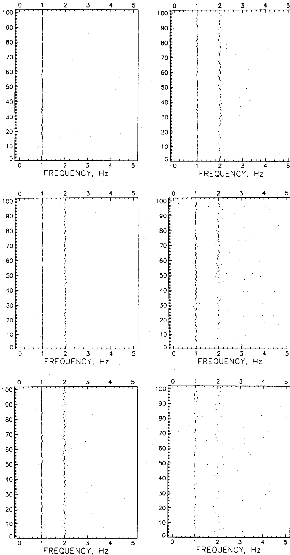
Fig. 2 20%-noise results at various values of ORDER (the number of retained singular values). All identified frequencies with Modal Amplitude Coherence of at least 10% are shown.
