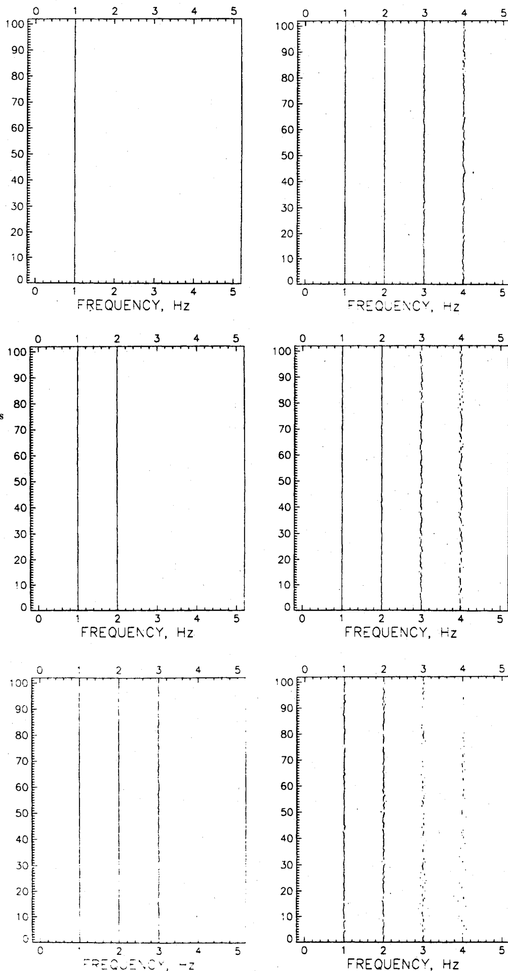
Fig. 3 1%-noise results at various values of ORDER (the number of retained singular values). All identified frequencies with Modal Amplitude Coherence of at least 10% are shown.
