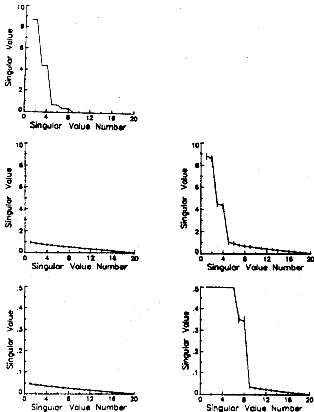
Fig. 1 Singular value spectra for simulated data sets. Vertical lines show extent of scatter in each Monte Carlo analysis.
